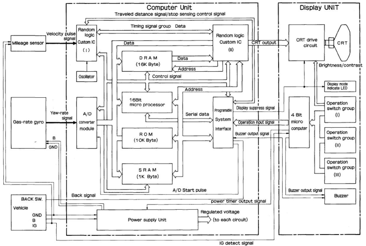
Fig. 1: System configuration diagram of "Electro Gyro-Cator",
